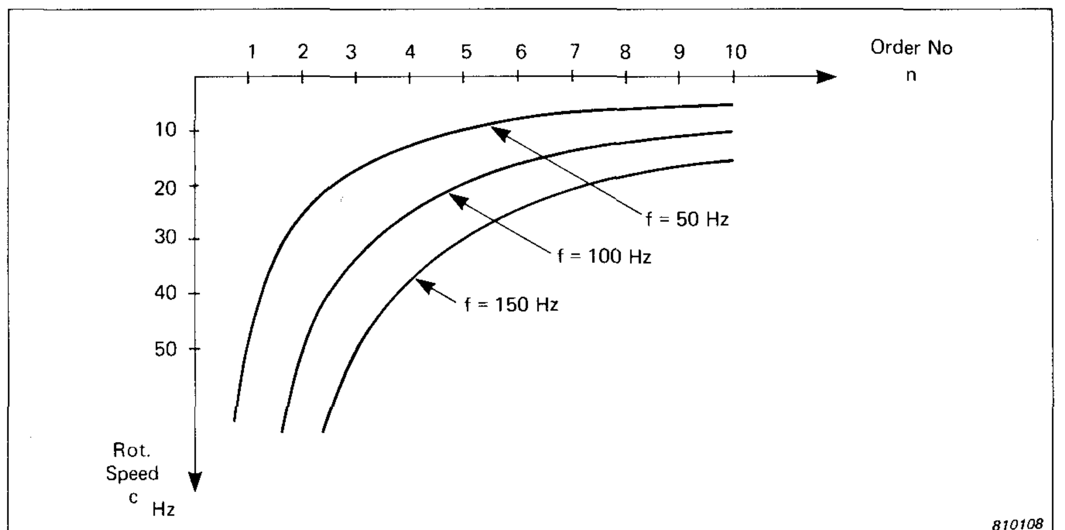
Fig. 6. Constant frequency curves
