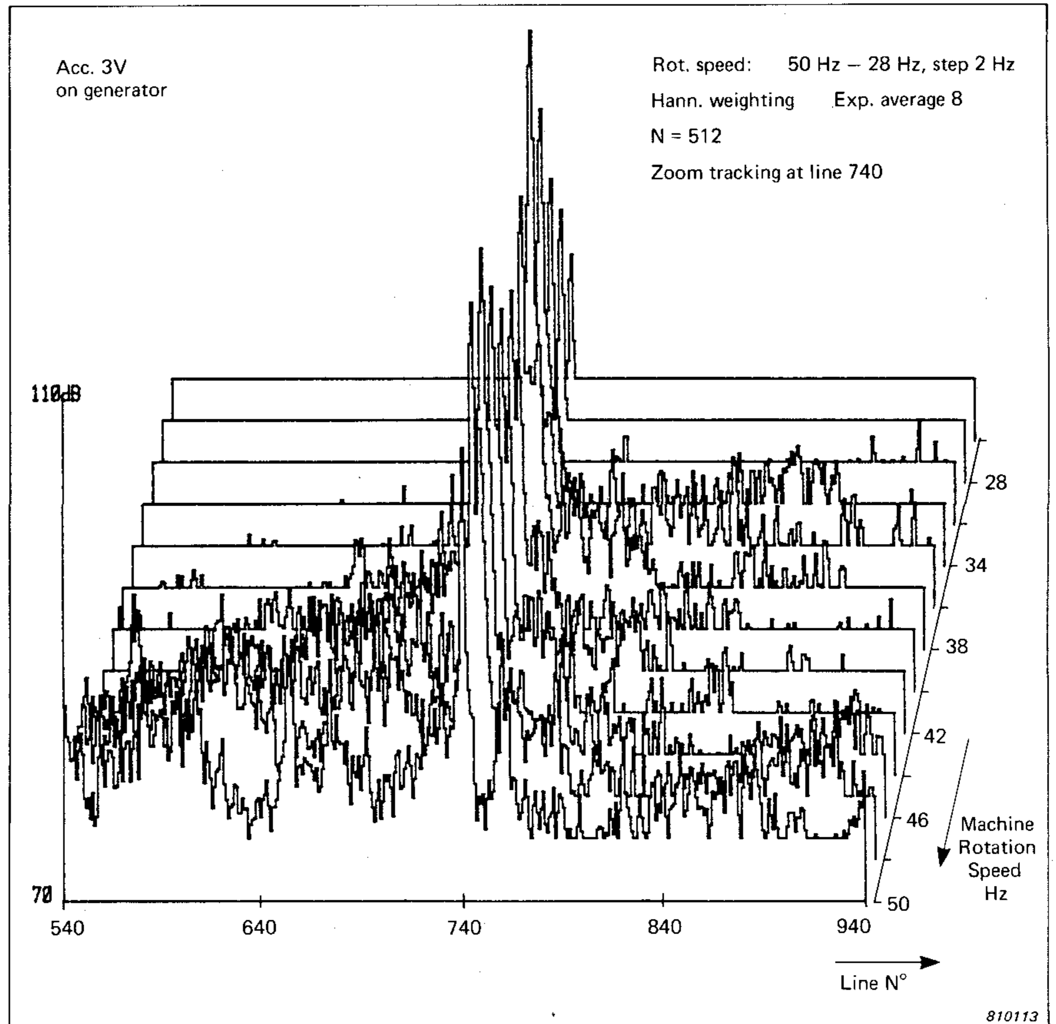
Fig.10. 400 line zoomed order analysis around the 37. harmonic (line 740) during rundown
