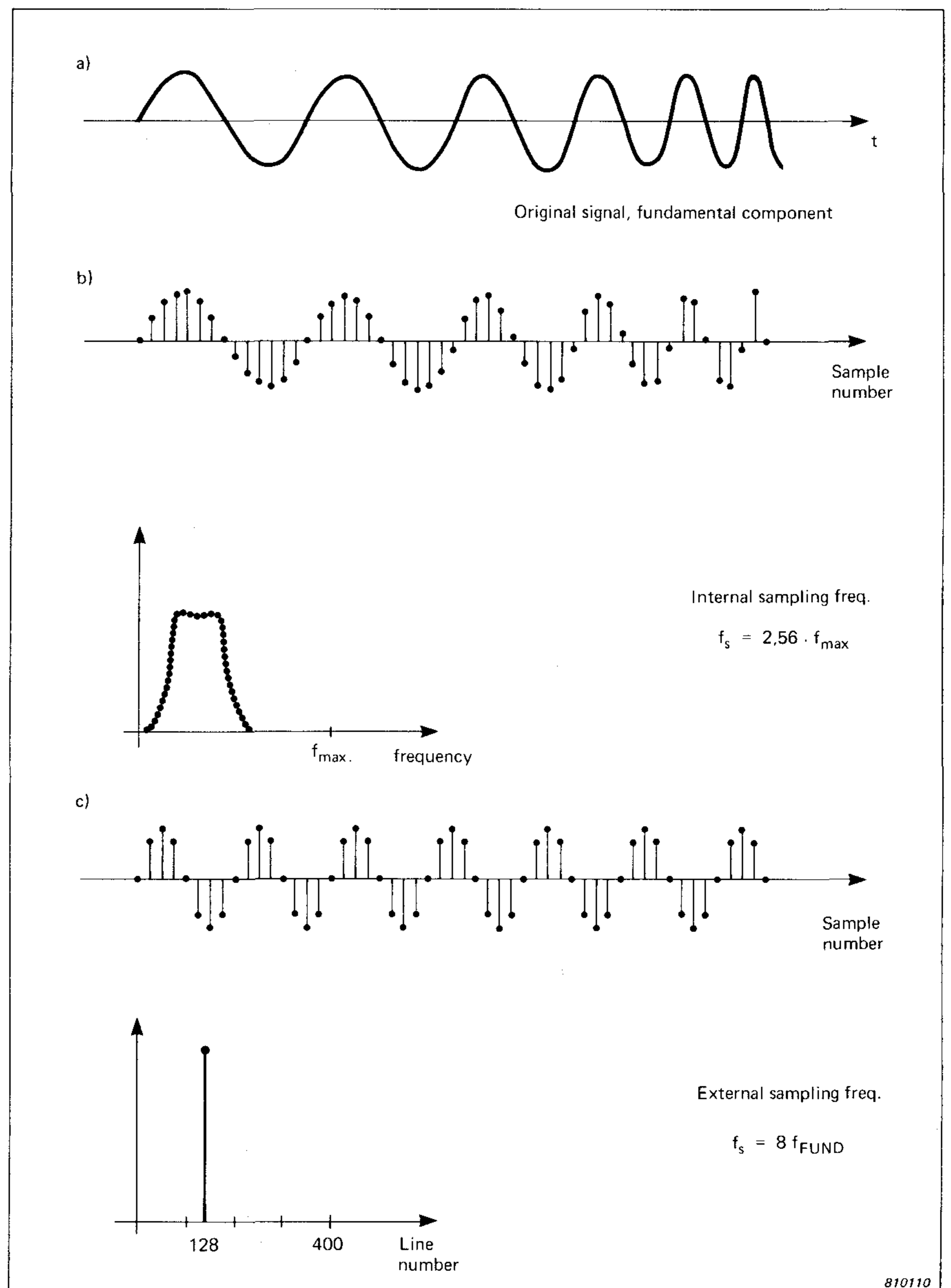
Fig.2. Principle in order analysis
