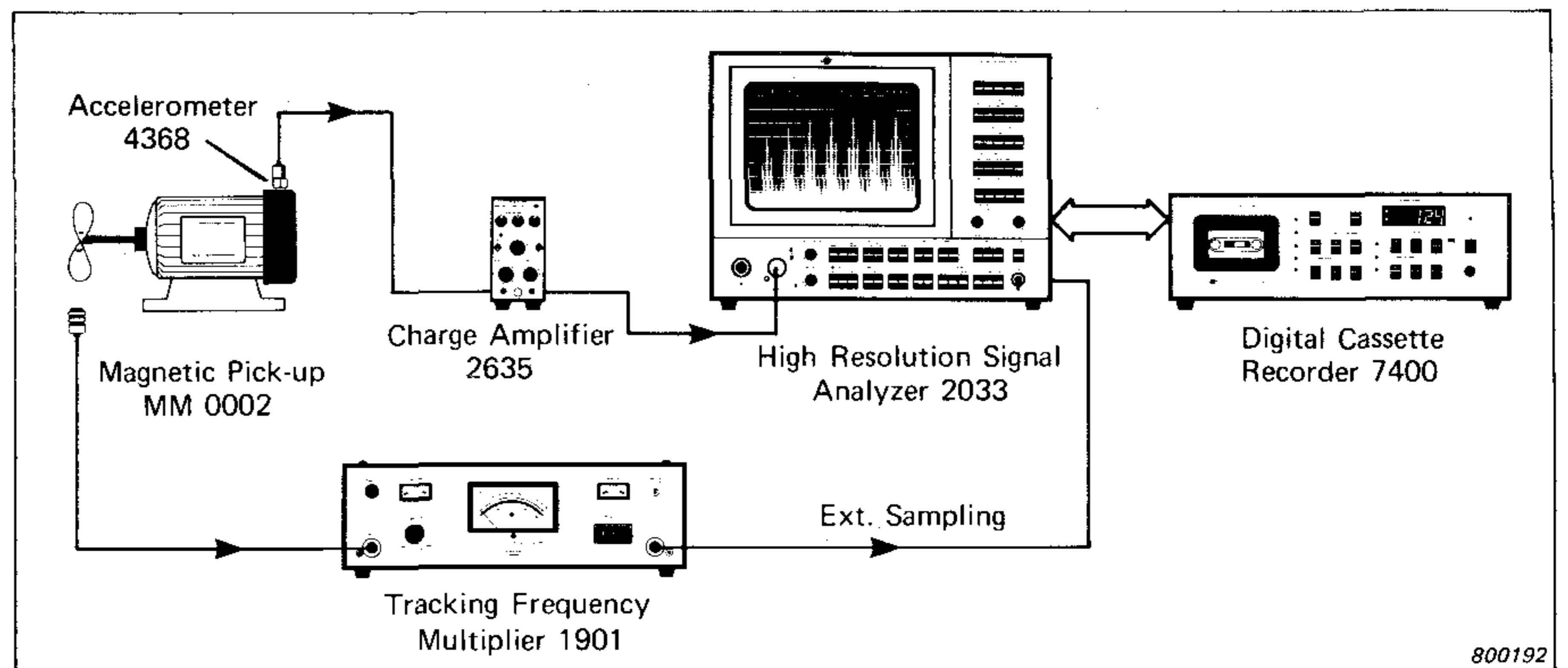
Fig.1. Instrumental set-up for order analysis
