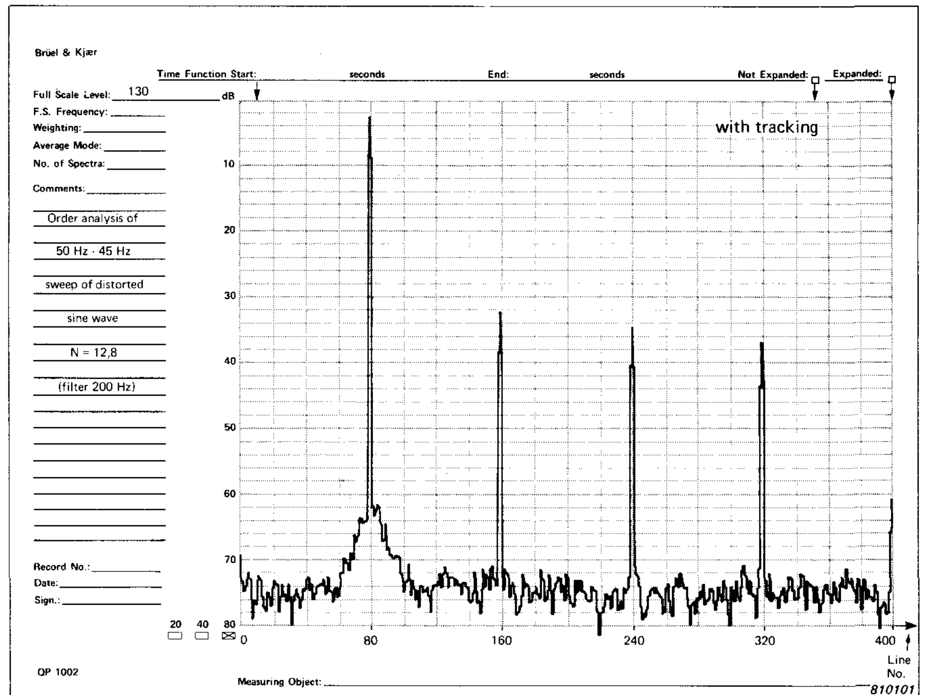
Fig. 3. Analysis of first 4 harmonics of a 50 Hz to 45 Hz sweep of a distorted sinewave a) with internal sampling b) with external sampling
