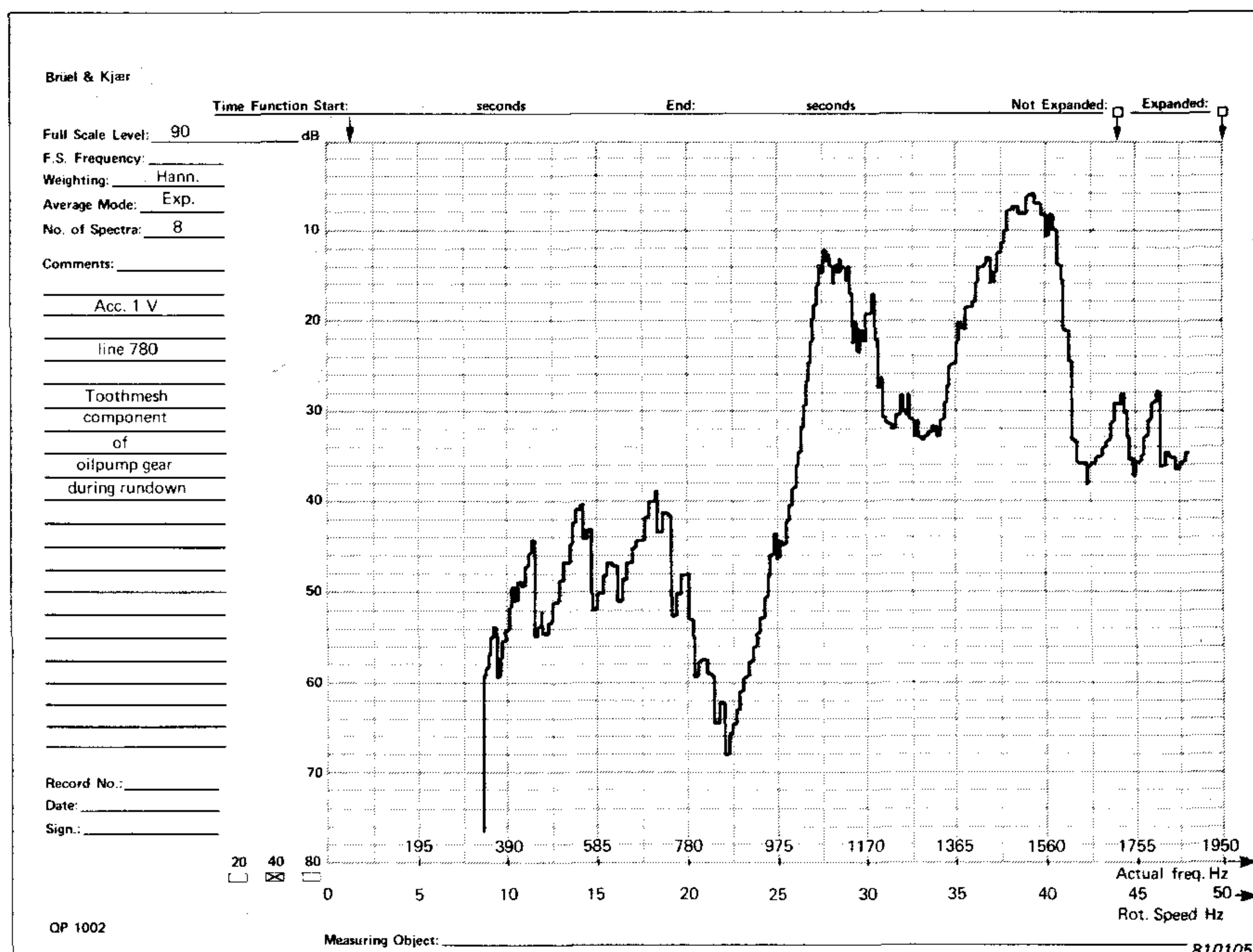
Fig.9. Toothmesh component of oil pump gear during rundown
