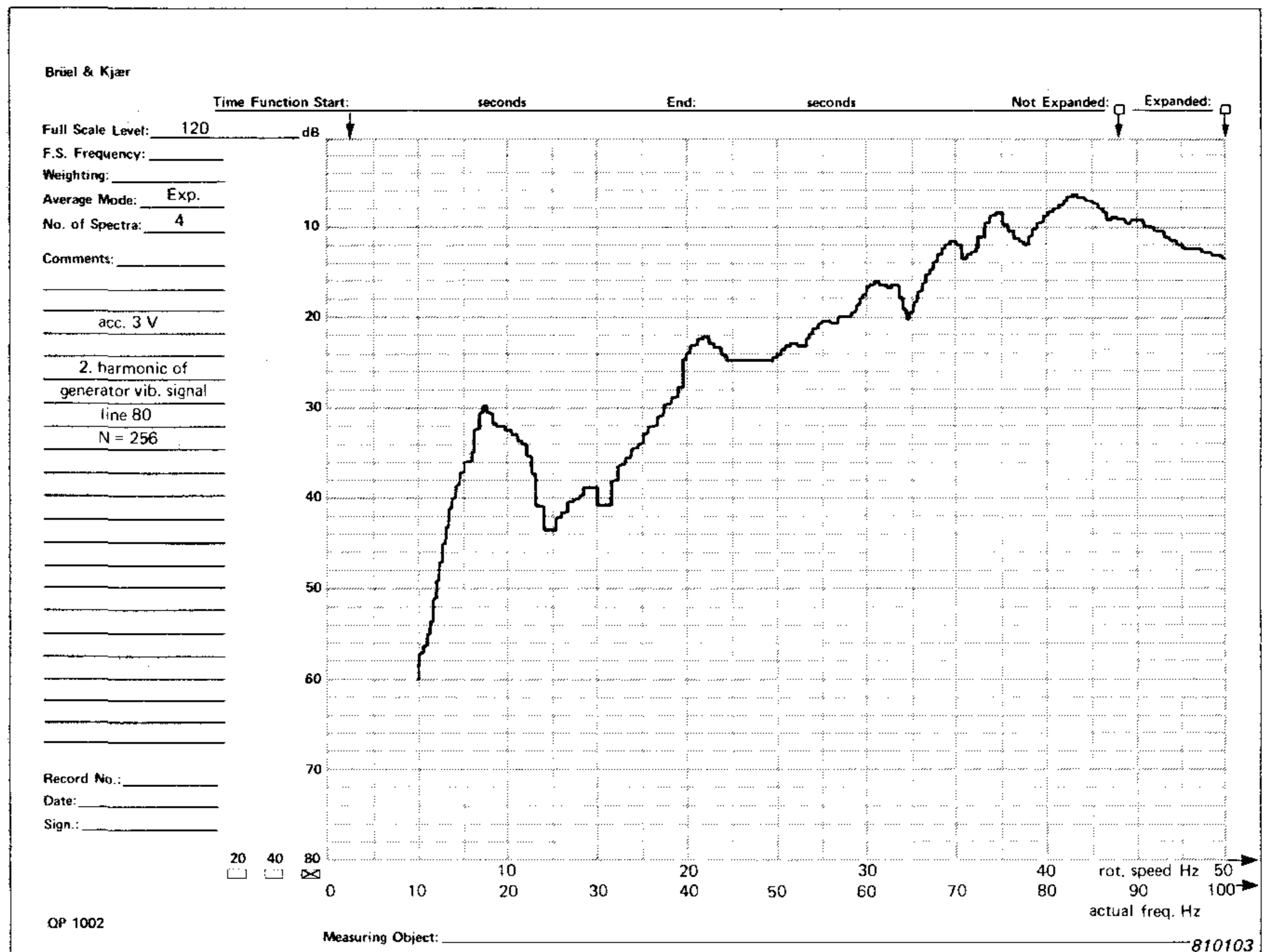
Fig.7. a) Fundamental of generator vibration signal during rundown b) 2. harmonic of generator vibration signal during rundown
